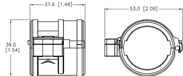
OPENED VIEW OF LOCKOUT DEVICE
